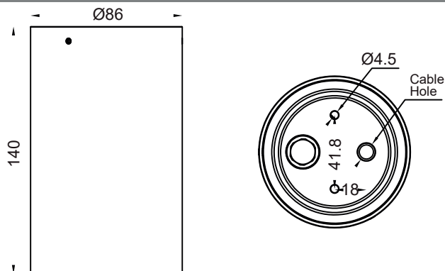
Physical Dimension(MM)
