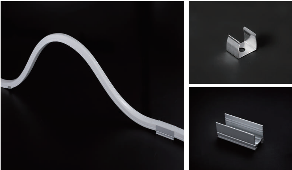
Stainless Clips Item No.: JK0026 Dimension(LxWxH): 10 x 12.8 x 13mm Material: SUS304\SUS316
